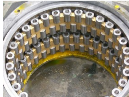
ROLLER BEARINGS
